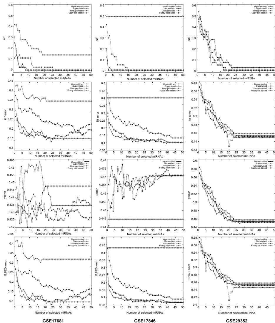
Figure 4 Error rates of the SVM obtained using different discretization methods averaged over 50 random splits. Abbreviations: SVM, support vector machine; miRNA, microRNA; AE, apparent error; BI, bootstrap error; \gamma , no-information error; B.632+, B.632+ error.
