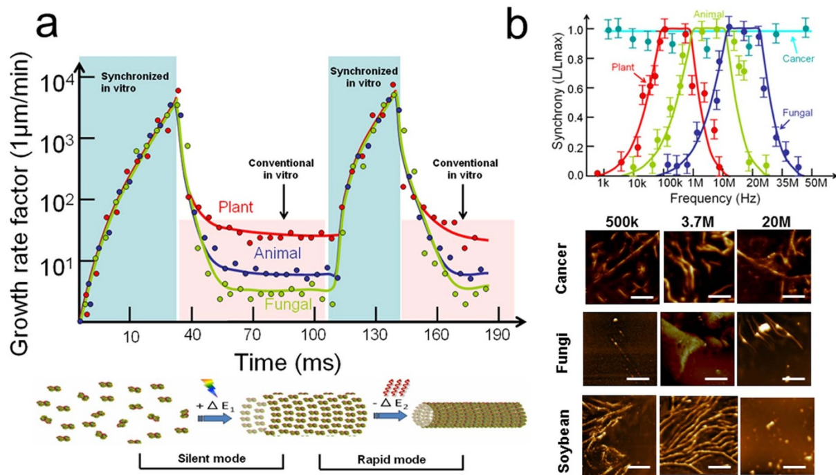
Figure 4 | Tubulins share electromagnetic frequency band in a complementary manner: (A). We have plotted growth factor (how many times the 1\mu\text{m}/\text{min} ) during synchronized in vitro for three species. Sudden fall is the point where several drugs were added, growth returns the specific features observed in conventional in vitro process. Then, the more tubulin is added to supersede the drug effect and remove noise, as soon as synchrony is established, high growth returns, the difference between three species disappears. Below the plot, we schematically present our model, during silent mode, due to synchrony the cylindrical form is produced, then it absorbs energy, and afterwards rapid assembly starts which releases energy, this is the rapid mode. (B). We plot ratio of the maximum average length \langle L \rangle to the maximum length \langle L_{\text{max}} \rangle measured from the AFM chip as a function of frequency for all drugs and for all species put together. For three samples, MCF7 breast cancer cells, Fungi, and Soybean tubulins, we show AFM images when the chips were pumped with 500 kHz, 3.7 MHz, and 20 MHz ac signals respectively. The scale bar is 10\mu\text{m} .
