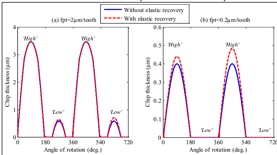
Figure 12. Effect of elastic recovery on instantaneous uncut chip thickness
