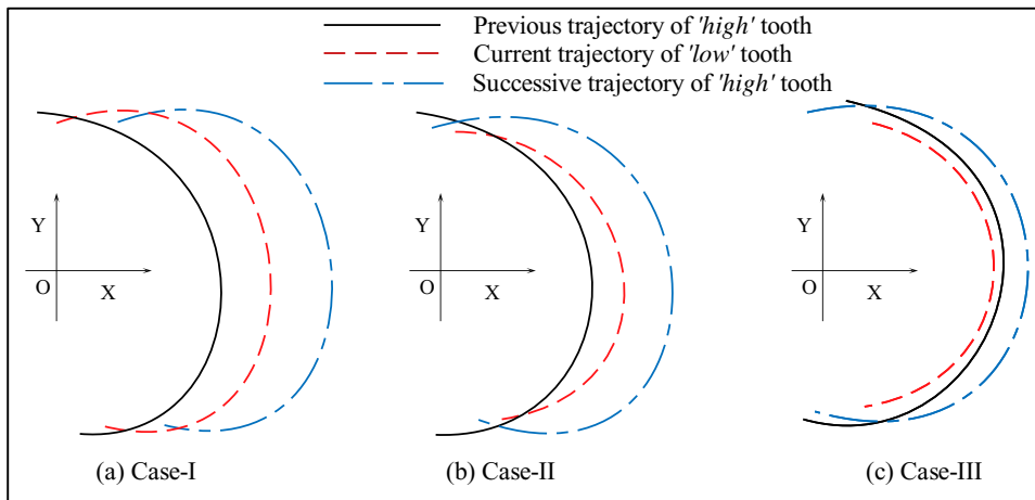
Figure 1. Interaction of cutting edge trajectories in the presence of cutter runout.
