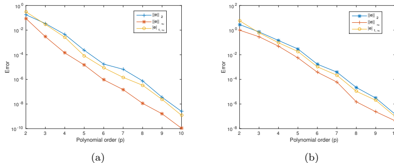
Figure 7: Error vs. p for (a) Case 1 (b) Case 2.
