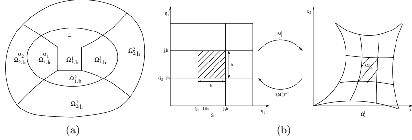
Figure 2: (a) Discretization, (b) Mesh imposing on \Omega_i, i = 1, 2 .
