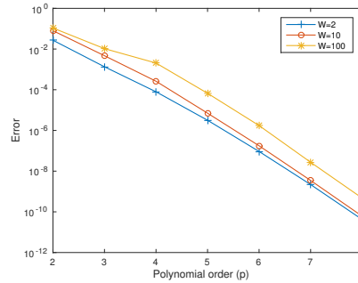
Figure 5: \|e\|_2 vs. p for p -version method.
