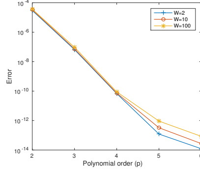
Figure 4: \|e\|_2 vs. p for p -version method.
