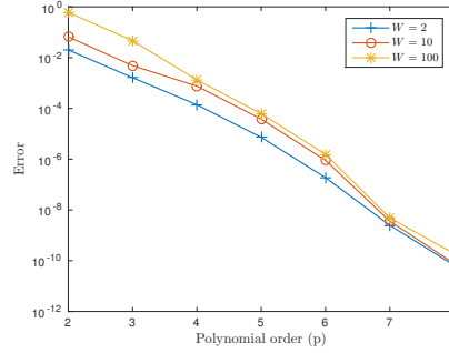
Figure 6: \|e\|_2 vs. p for p -version method.
