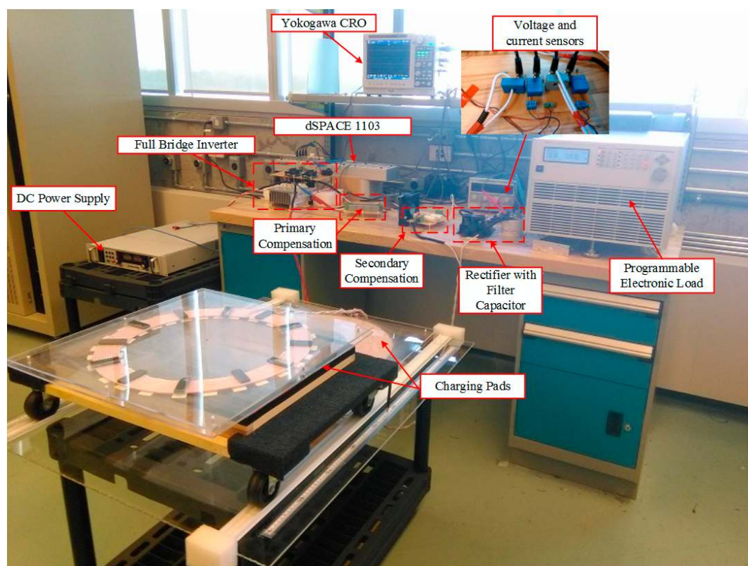
Figure 8. Experimental setup.
