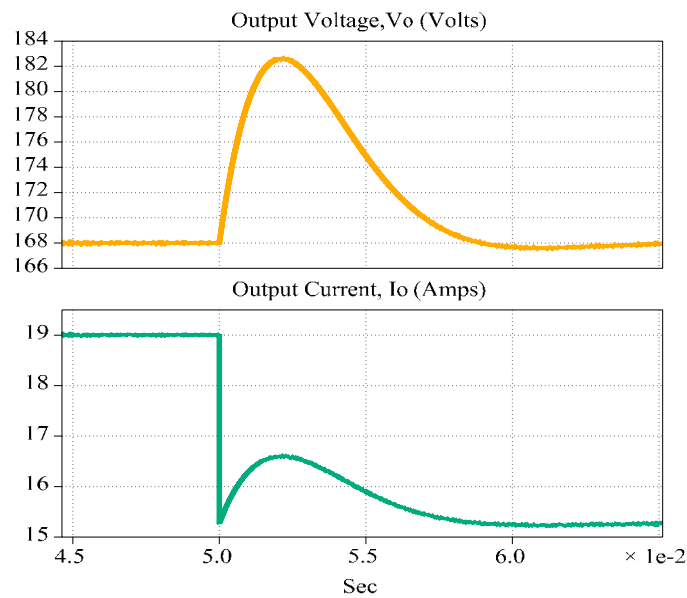
Figure 9. Simulation results for step change in load.
