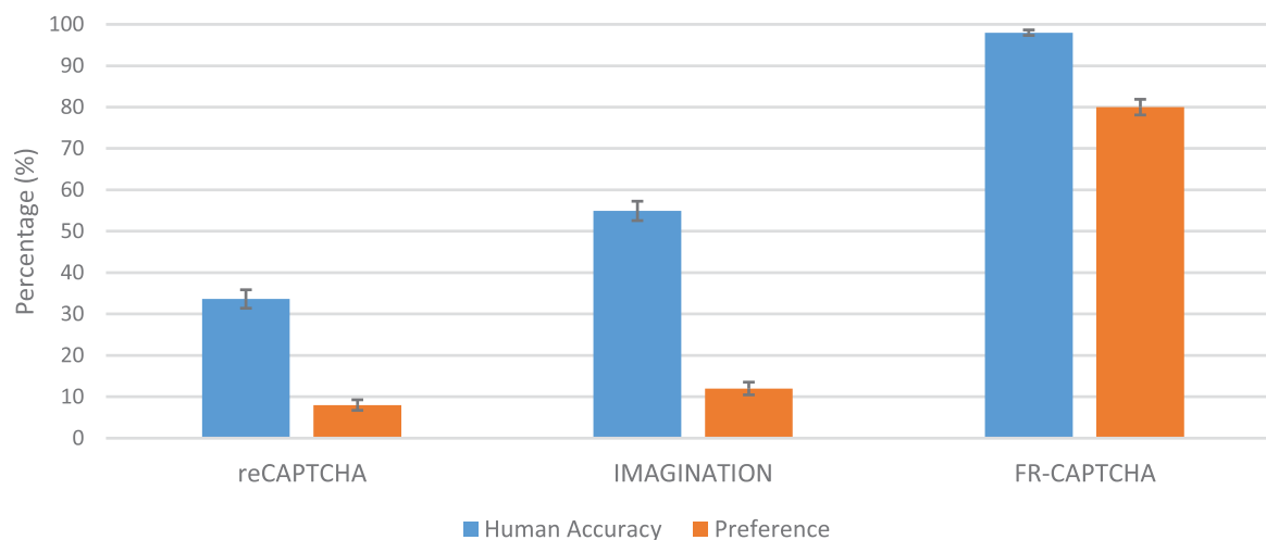
Figure 6. Human performance and preference on reCAPTCHA, IMAGINATION and the proposed FR-CAPTCHA. Based on 2,997 responses, the proposed CAPTCHA achieves higher human performance and is also preferred by majority (80%) of the users. The error bars represent confidence intervals.
