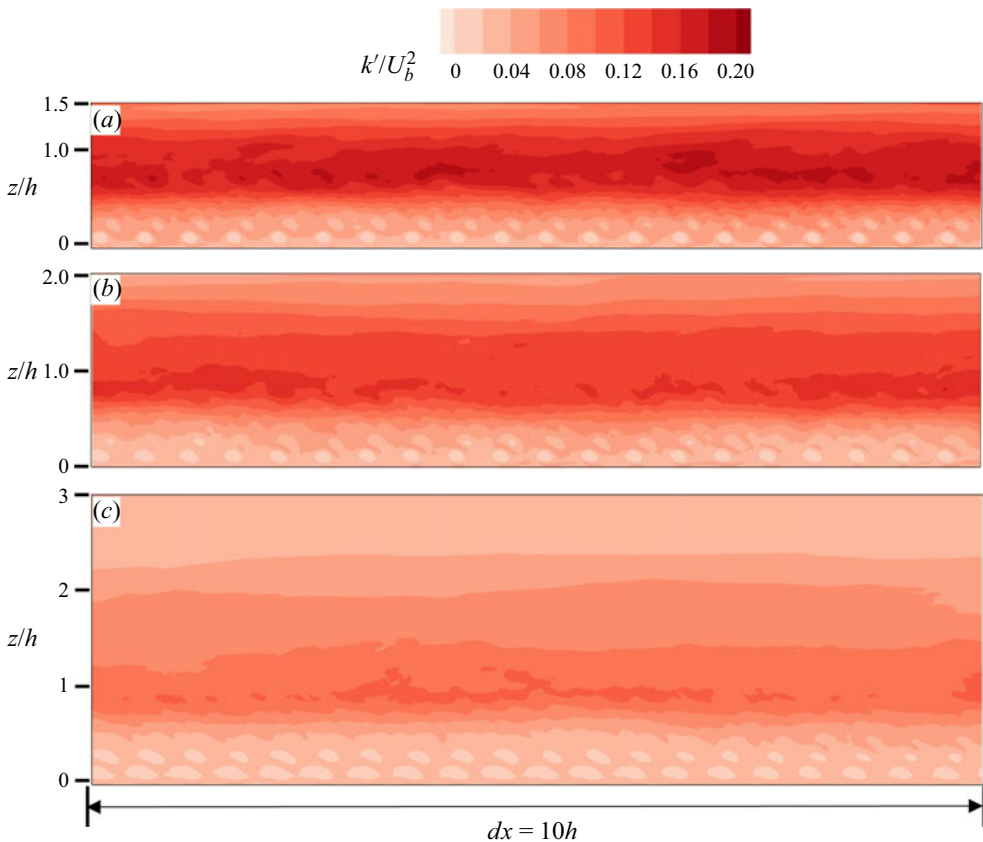
Figure 27. Distributions of the TKE in (a) case 1, (b) case 10 and (c) case 11 in the xz plane with y/h=0 , where the centre line of plant nos 101–200 is located at a streamwise distance of dx=10h . The relative submergence H/h gradually increases from (a) to (c).
