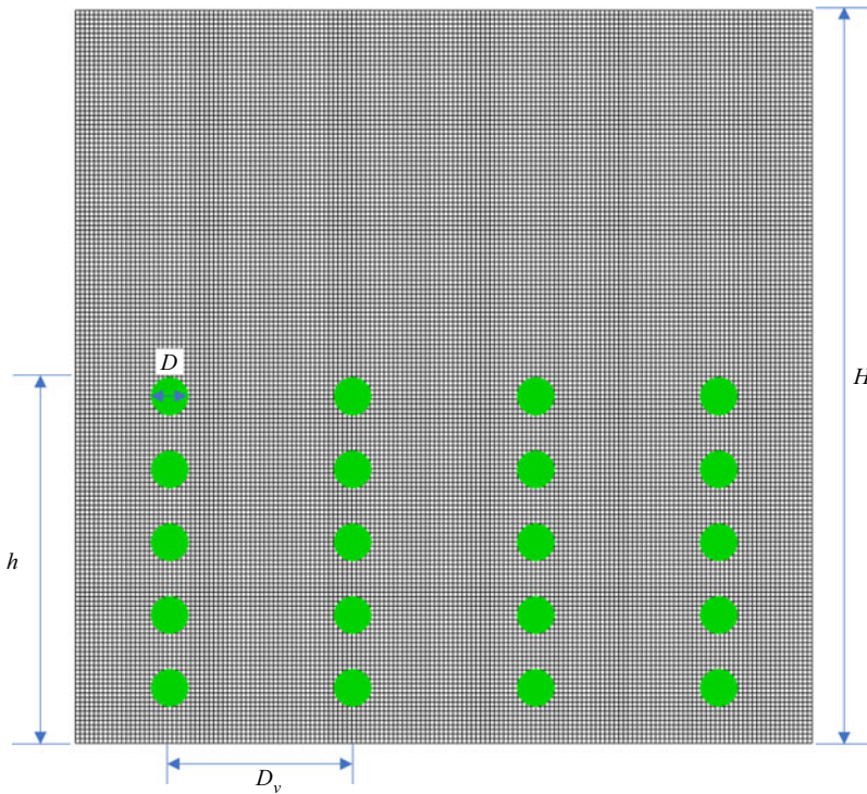
Figure 4. The plane projection of the meshing part of the computational domain of the C1 case (see table 1 ). This area contains five single plants. The side length of the grid is L_g = 0.0125h , and the IBM unit diameter is D = 0.1h . For three different submergences, the flow depths are H = 1.5h , 2h and 3h , respectively.
