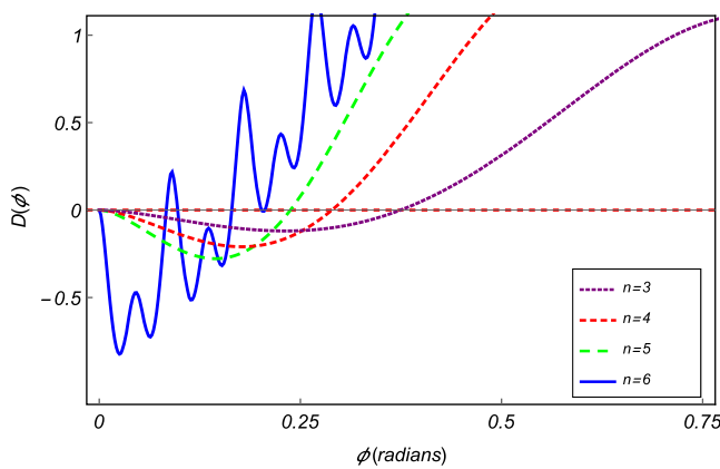
Fig. 3 Information difference \mathcal{D}^{[n]}(\phi) plotted against dimensionless parameter \phi for different values of n , the number of observations made on the system. The left and right panels correspond to the two and three flavor cases, in vacuum, respectively. It is clear that, as the number of measurements n increases, the information difference becomes more
