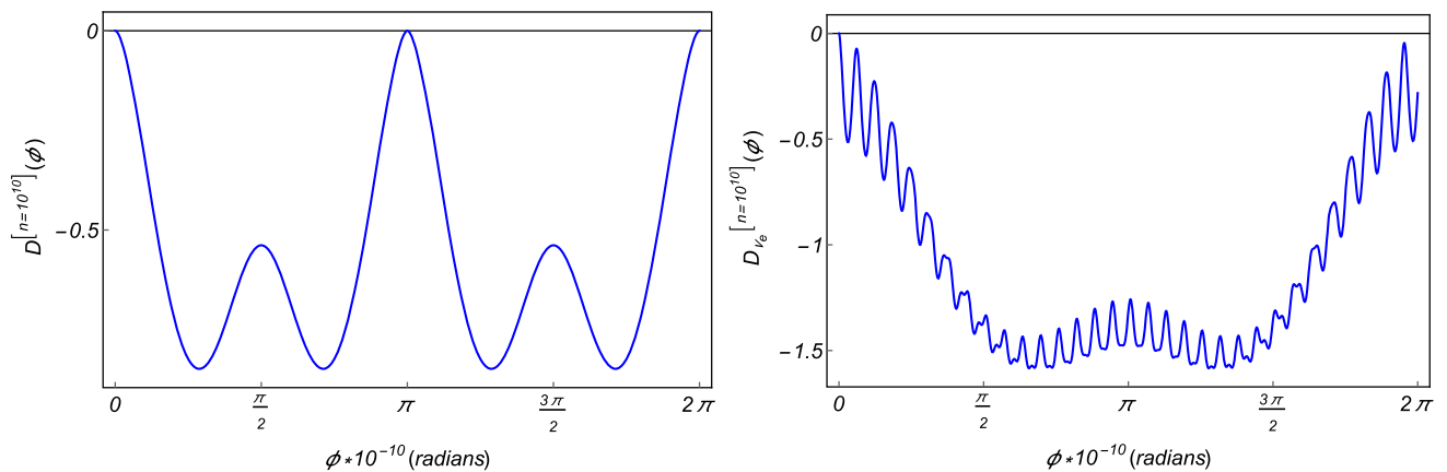
Fig. 8 Showing the the variation of the information deficit with the dimensionless parameter \phi \left( = \frac{\Delta_{21}L}{2\hbar cE} \right) , for n \approx 10^{10} in two (left) and three (right) flavor scenario of neutrino oscillations in vacuum. In three
