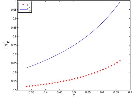
Figure 1: Comparison of maximal singlet fraction F^* and upper bound on singlet fraction F_D^* obtained using Dembo's bound
