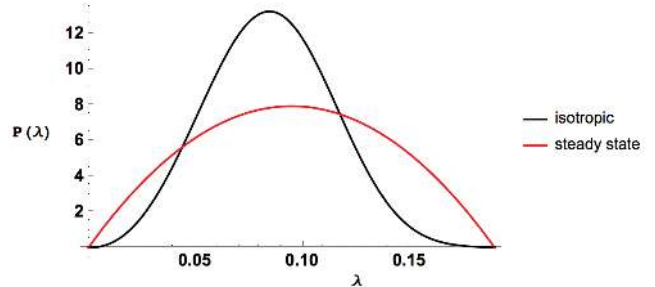
FIG. 5. Plots of the isotropic Weibull distribution and the Steady State distribution assuming that the new eigenvalues are equally distributed between \lambda = 0 and \lambda = \lambda_{max} . The distributions have been chosen so that \langle\lambda\rangle_{iso} = \langle\lambda\rangle_{ss} .
