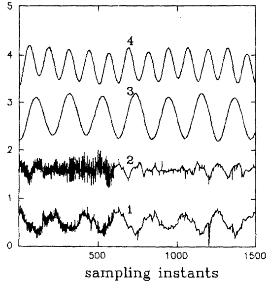
Fig. 4. Training data generated by tracking sinusoid trajectories: 1) torque input at joint 1; 2) torque input at joint 2; 3) joint 1 position; and 4) joint 2 position. (Input/output data are normalized and scaled differently.)
