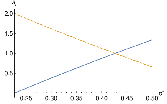
FIG. 1. (Color online) Eigenvalue \lambda_I (dashed, red line) and \lambda_Z (bold, blue line) for the intermediate map Choi matrix of the non-Markovian dephasing channel characterized by Eq. (5). The intermediate p -range lies between p:=p_* and p:=p^* , where p_* < \alpha_- , and p^* is varied over the interval [p_*, \frac{1}{2}] . At p^*:=p_* , \lambda_I = 2 and \lambda_Z = 0 . At p^* = \alpha_- , the eigenvalues crossover, i.e., \lambda_I = \lambda_Z = 1 , and furthermore the channel becomes maximally dephasing, i.e., \kappa = \frac{1}{2} in Eq. (5). Here, \alpha := 0.3 and p_* := \alpha_- - 0.2 \approx 0.23 .
