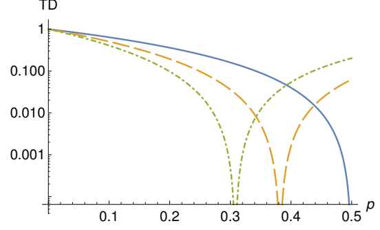
FIG. 5. Log plot of trace distance TD between \rho_0 \equiv \mathcal{E}(|\psi_0\rangle\langle\psi_0|) and \rho_1 \equiv \mathcal{E}(|\psi_1\rangle\langle\psi_1|) as a function of p with \theta := \frac{\pi}{2} , under the considered non-Markovian dephasing noise. The bold (blue) curve represents Markovian dephasing, and shows no recurrence. The dashed (red, \alpha = 0.5 ) and dot-dashed (green, \alpha = 0.9 ) show enhanced distinguishability beyond their respective crossover point \alpha_- , indicative of non-Markovianity. Note that larger \alpha shows a larger enhancement region, suggesting larger non-Markovianity in the sense of BLP [33].
