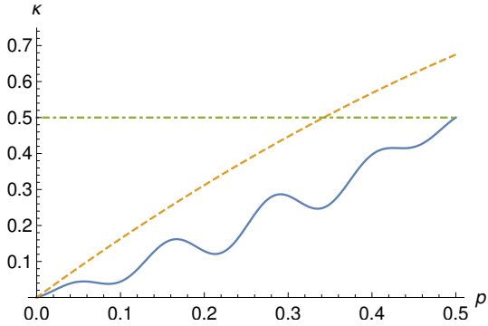
FIG. 6. Plot of \kappa(p) in Eq. (25) as a function of p , with \eta = \frac{1}{2} and \omega = 50 (bold, blue line). This dephasing channel corresponds to the first case of Eq. (24) and non-Markovianity arises from regions of negative slope in the plot. The dashed (red) line corresponds to the non-Markovian dephasing Eq. (5) with \alpha = 0.7 . The mixing rate d\kappa/dp is never negative, and non-Markovianity pertains to the first case in Eq. (24).
