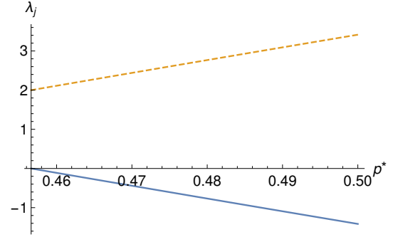
FIG. 2. (Color online) Eigenvalue \lambda_I (dashed, red line) and \lambda_Z (bold, blue line) for the intermediate map Choi matrix of the non-Markovian dephasing channel characterized by Eq. (5). The intermediate p -range lies between p:=p_* and p:=p^* , where \frac{1}{2} > p_* > \alpha_- , and p^* is varied over the interval [p_*, \frac{1}{2}] . For p^* > p_* , one finds \lambda_Z < 0 . Thus, the whole range p^* \in (p_*, \frac{1}{2}] corresponds to an NCP map, demonstrating the non-Markovianity of the channel characterized by Eq. (5). Here \alpha := 0.3 and p_* := \alpha_- + 0.03 \approx 0.46 .
