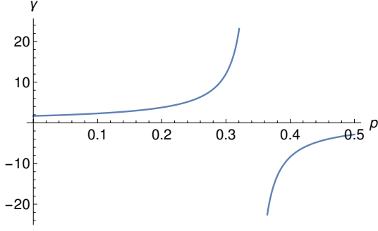
FIG. 3. Plot of the decoherence rate \gamma as a function of p for \alpha = 0.7 . Note the singularity at \alpha_- ( \approx 0.34 ), just after which \gamma becomes negative, indicating that the evolution is non-Markovian.
