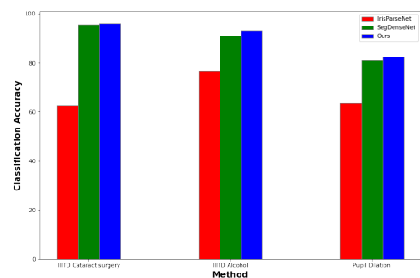
Fig. 10: Showcasing the classification accuracy of existing and proposed segmentation methods on the datasets used in the paper.
