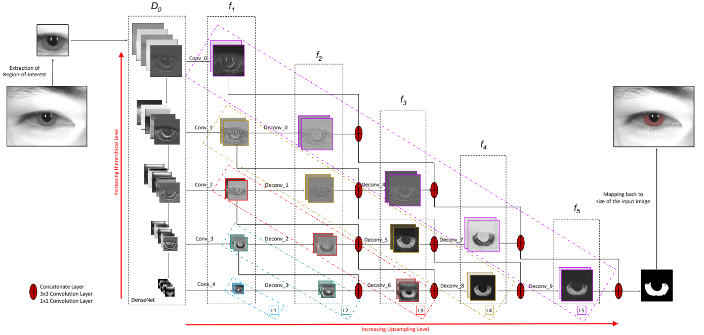
Fig. 4: Presents the proposed architecture, PyramidNet for iris and pupil segmentation in an unconstrained environment. The dotted boxes represent the pyramid structure. The upsampling level increases in the x-direction, and the hierarchical level increases in the y-direction. The intermediate feature maps in L1-L5 levels present the different information stored in each map which results in preserving the fine and the global structure of the iris and pupil in the final output. (Best viewed in color)
