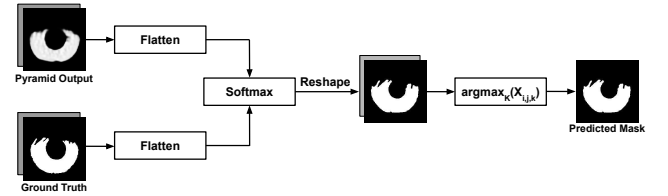
Fig. 6: Illustrating the process of calculating the loss that is back-propagated through the segmentation network.
