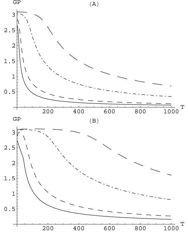
Fig. 4. GP (in radians) vs temperature ( T , in units where \hbar \equiv k_B \equiv 1 ) from Eq. (28). Here \omega = 1.0 , \theta_0 = \pi/2 , the large-dashed, dot-dashed, small-dashed and solid curves, represent, respectively, \gamma_0 = 0.005 , 0.01 , 0.03 and 0.05 . (A) squeezing is set to zero; (B) squeezing non-vanishing, with r = 0.4 and \Phi = 0 .
