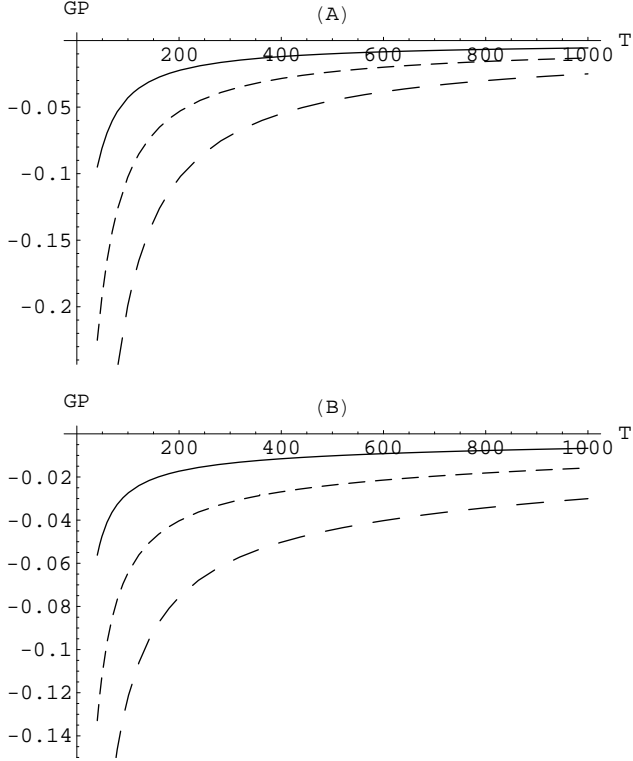
Fig. 2. GP (in radians) as a function of temperature ( T , in units where \hbar \equiv k_B \equiv 1 ) for QND interaction with a bath of harmonic oscillators (Eq. (14)). (A) with \gamma_0 = 0.005 and vanishing squeezing. The solid, dashed and larger-dashed lines correspond to \theta_0 = \pi/8, 3\pi/16 and \pi/4 . (B) Same as Figure (A), except that here squeezing is non-vanishing, with r = 0.7 and a = 0.1 .
