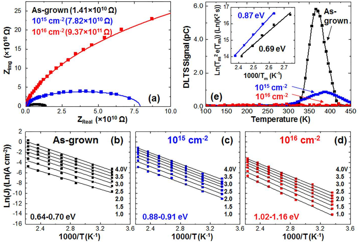
Figure 2. a) Nyquist plots ( Z_{\text{img}} vs. Z_{\text{Real}} ) for heterostructures ion bombarded with various \text{He}^{2+} dosages suggesting a single transport mechanism dominated by the bulk of the film with increasing resistance (extracted from the intercept of the semicircles on the real axis) with increasing dosage. Arrhenius plots of \ln(J) versus 1000/T at different voltages for b) as-grown (no bombardment), c) 10^{15} \text{ cm}^{-2} , and d) 10^{16} \text{ cm}^{-2} heterostructures. The activation energies (noted) are extracted from the slope of the linear fits. Range of activation energies corresponds to small variation in the slope of the linear fits at different voltages. e) DLTS signal measured at the same rate window (80-160 ms) for heterostructures bombarded with various \text{He}^{2+} dosages. Inset shows the Arrhenius plot of \ln(\frac{T_m^2}{e(T_m)}) versus \frac{1000}{T_m} , where T_m is the temperature at which maximum of a DLTS peak, obtained in a rate window between t_1 and t_2 . e(T_m) is the emission rate of a defect with DLTS peak located at T_m . The activation energy of each trap state ( E_d ) can be extracted from the slope of the linear fits.
