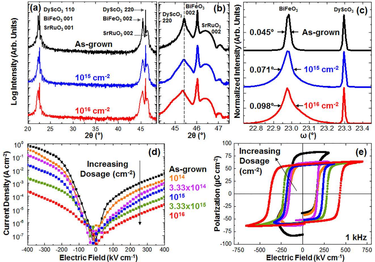
Figure 1. a) Wide angle 2\theta - \omega X-ray diffraction scans and b) zoom-in about the 002- and 220-diffraction conditions for heterostructures ion-bombarded with various He 2+ dosages. c) Rocking curves for heterostructures ion-bombarded with various He 2+ dosages obtained about the 002-diffraction conditions of film and substrate. d) Leakage current density as a function of DC electric field, and e) ferroelectric polarization-electric field hysteresis loops measured at 1 kHz after ion bombardment with various He 2+ dosages.
