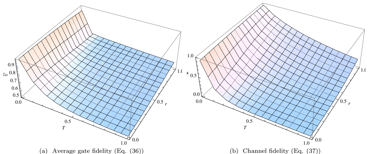
FIG. 2: SGAD channel properties, as function of temperature ( T ) and squeezing, parametrized by r , with time t = 0.5 , frequency \omega = 0.01 , bath parameter \gamma_0 = 0.1 and squeezing angle \Phi = 0.3 for (a) and \Phi = 0.0 for (b) (in the units where \hbar = k_B = 1 ). Both quantities show a counter-intuitive rise with squeezing.
