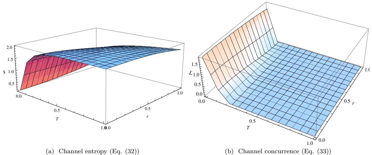
FIG. 1: Two possible quantifications of the decoherence due to the action of a SGAD channel, as function of temperature ( T ) and squeezing, parametrized by r , with time t = 0.5 , frequency \omega = 0.01 , bath parameter \gamma_0 = 0.1 and squeezing angle \Phi = 0.3 (in the units where \hbar = k_B = 1 ).
