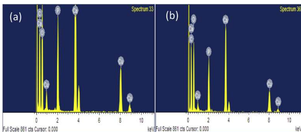
Fig. 6. EDX of (a) HAp and (b) DOX-HAp-PVA nanocomposite.
