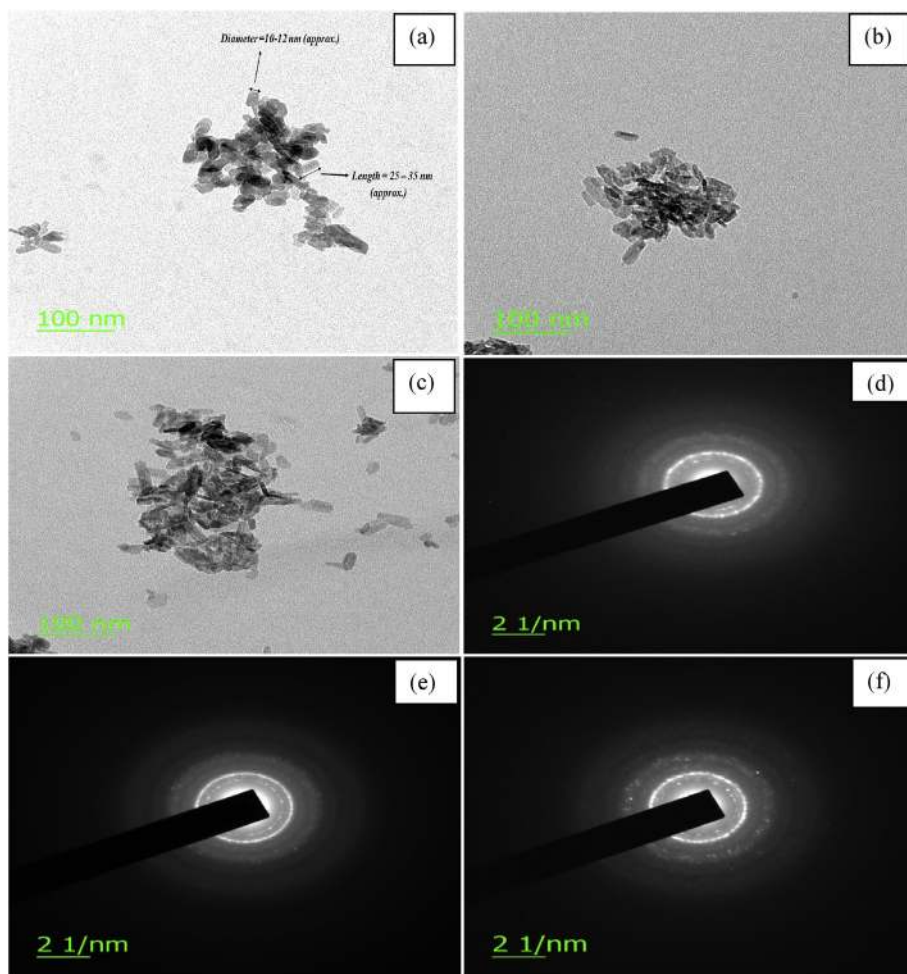
Fig. 4. TEM micrographs of (a) HAp powders, (b) DOX-HAp nanocomposite (c) DOX-HAp-PVA nanocomposite. Selected area electron diffraction (SAED) pattern of (d) HAp, (e) DOX-HAp nanocomposite, and (f) DOX-HAp-PVA nanocomposite.
