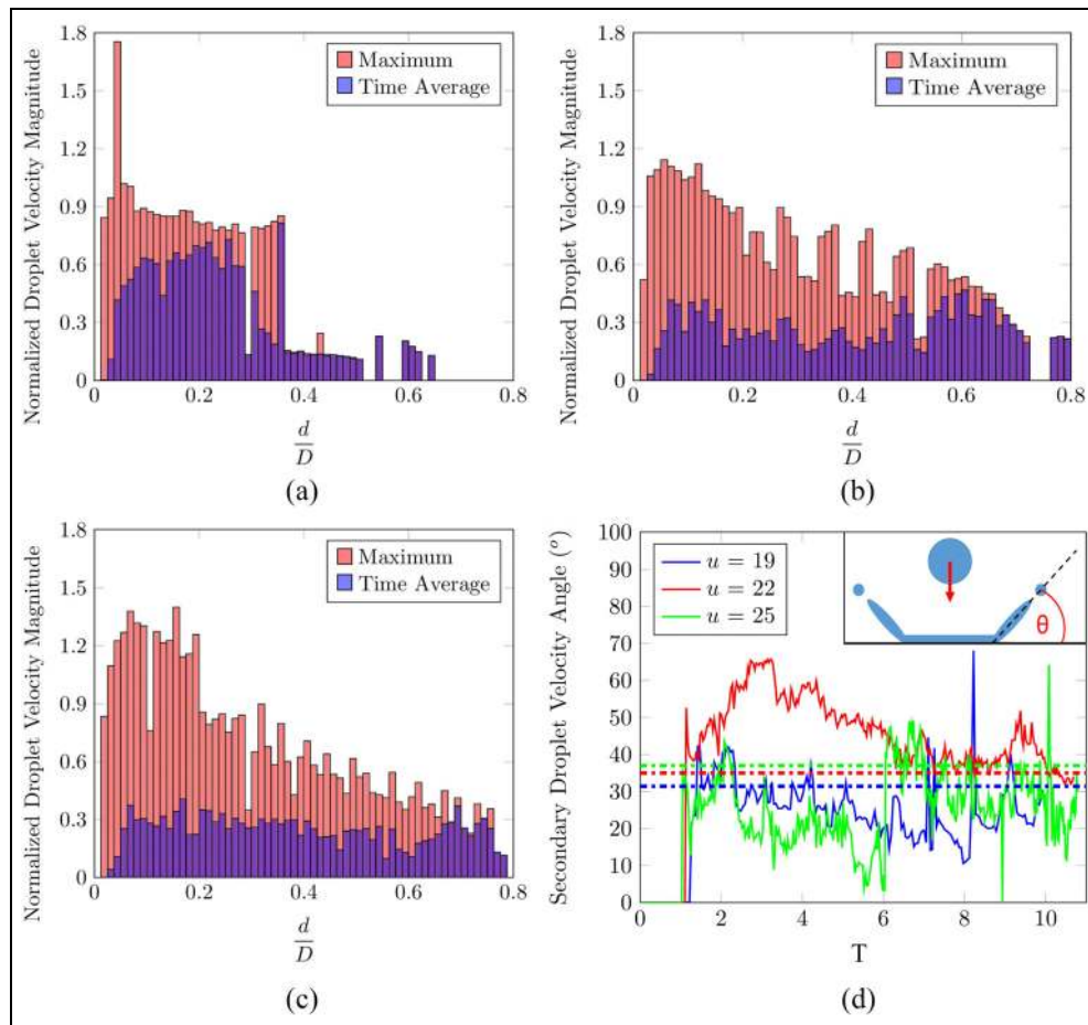
Figure 12. Maximum and time-averaged normalized secondary droplet velocities, defined as |\bar{U}|/V_0 , where V_0 is 10 m/s, as a function of dimensionless diameter for (a) u = 19 , (b) u = 22 and (c) u = 25 . (d) Average velocity angle with respect to horizontal of all secondary droplets as a function of dimensionless time. The dotted lines correspond to the predictions from Fredorchenko and Wang's 28 model for each case.
