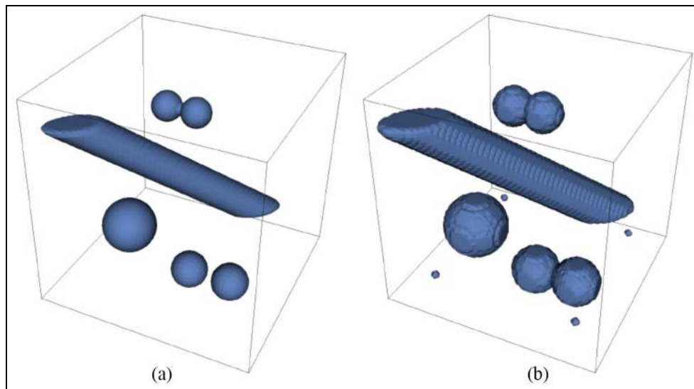
Figure 2. A sample test case used to validate the secondary droplet characterization algorithm: (a) visualized with an isovolume of 0.5 (regular visualization). (b) Visualized with an isovolume of 0.01 to capture the four underresolved droplets used to test the algorithm.
