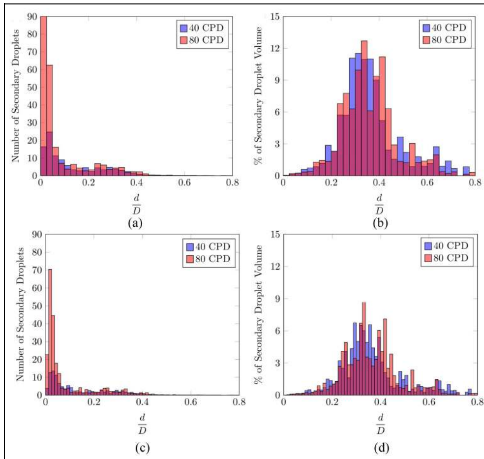
Figure 9. Secondary droplet distributions for the drop train impingement at u=22 with a bin size of 2.75\ \mu\text{m} (top row) and a bin size of 1.375\ \mu\text{m} (bottom row). In each subfigure, results from the simulation at 40 CPD (blue) and 80 CPD (red) are compared.
