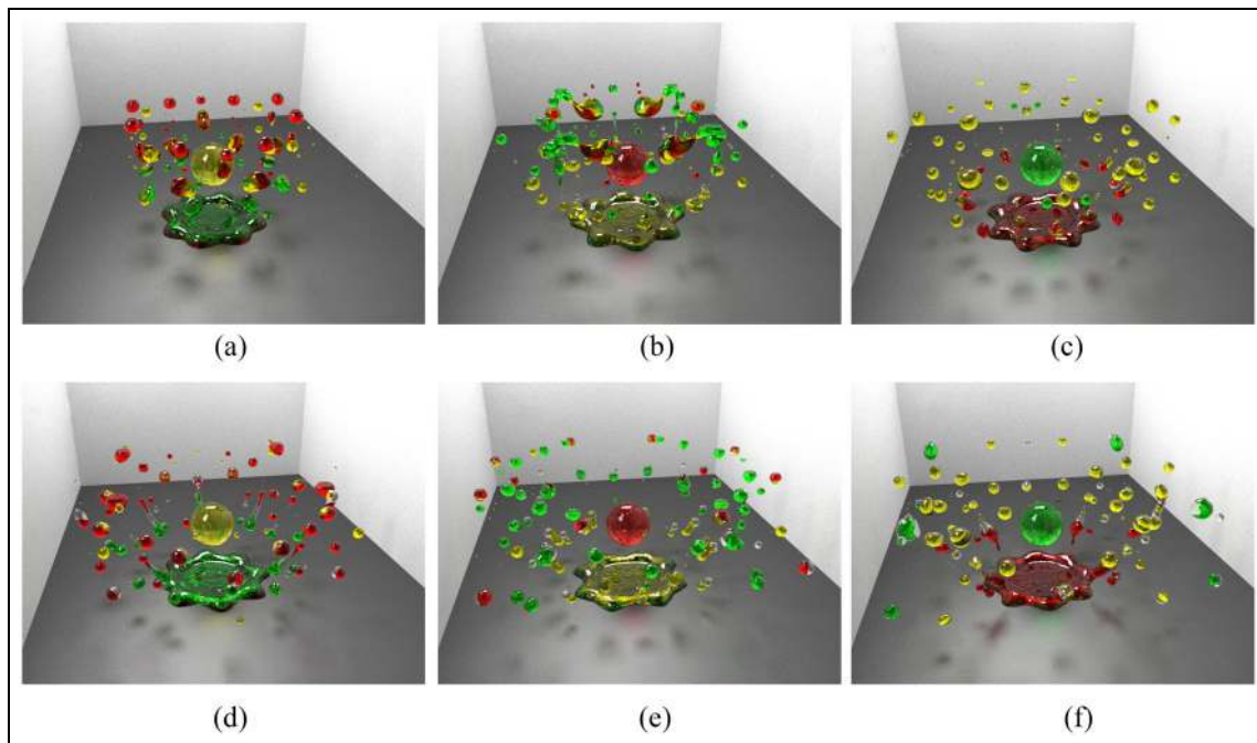
Figure 7. Simulation results for the ethanol drop train impingement case at u = 22 . Results are shown after the impingement of the third through eight drops, respectively: (a) T = 2.9 , (b) T = 3.9 , (c) T = 4.9 , (d) T = 5.9 , (e) T = 6.9 and (f) T = 7.9 . Note the similarity in secondary droplet distributions in (c–f), which indicate pseudo-steady state dynamics have been reached, while in (a) and (b) the early transient impingement dynamics are present resulting in a different secondary droplet distribution.
