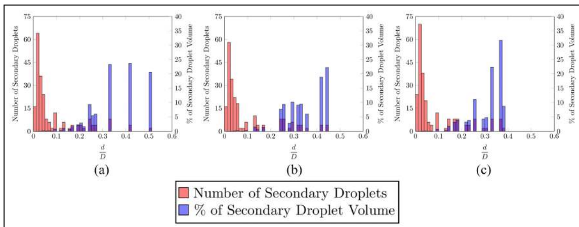
Figure 6. Temporal variation in the number of secondary droplets and percent of total secondary droplet volume as a function of dimensionless diameter, d/D , for the drop train impingement at u = 22 . Dimensionless times of (a) T = 5.172 , (b) 5.517 and (c) 5.862 correspond to the results shown in Figure 5(a)–(c), respectively.
