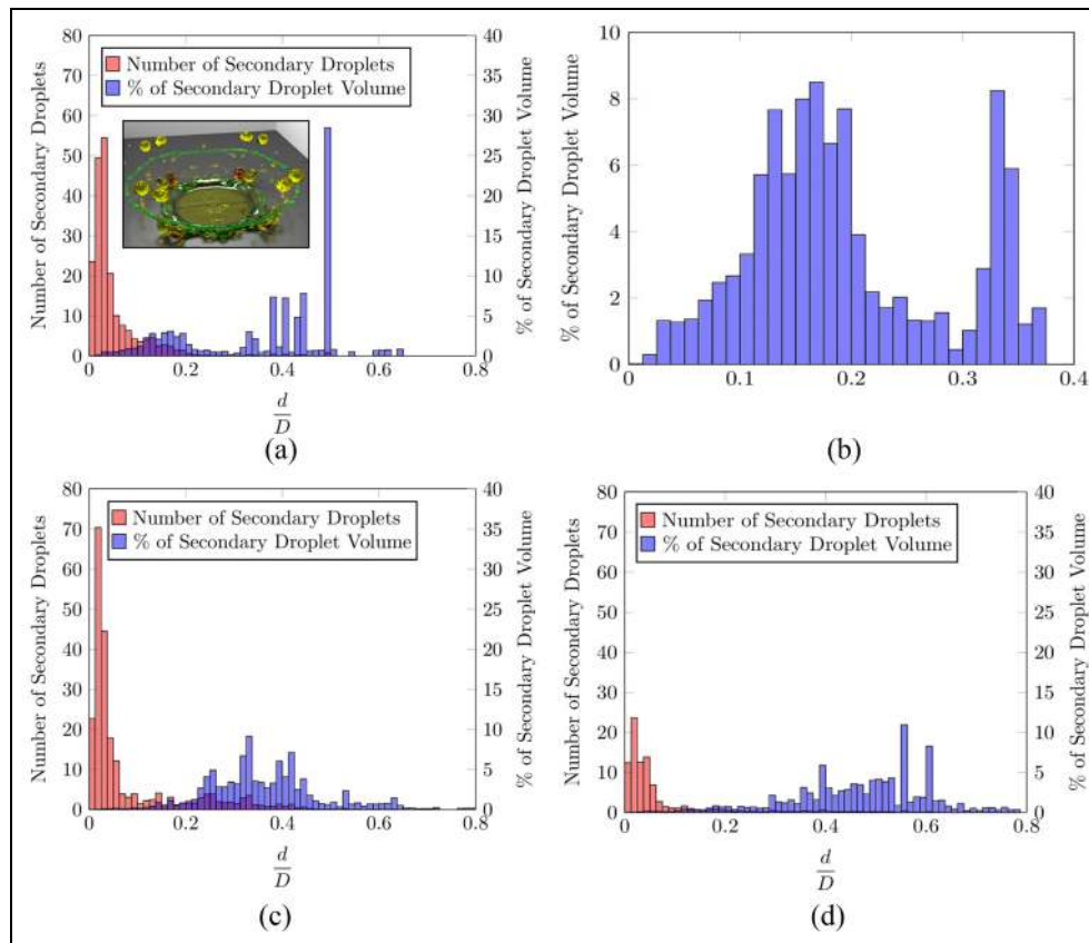
Figure 10. Time-averaged number of secondary droplets and percent of secondary droplet volume as a function of d/D for (a) u = 19 , with the inlay showing the large secondary droplets responsible for the peak in the percent of secondary droplet volume at d/D = 0.49 , (b) percent of secondary droplet volume at u = 19 , excluding the large secondary droplets seen in (a), (c) u = 22 and (d) u = 25 .
