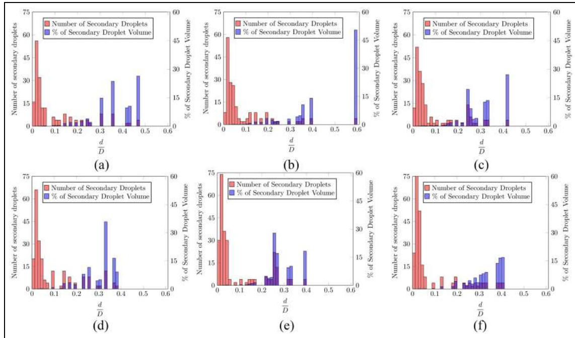
Figure 8. Instantaneous secondary droplet distributions from the ethanol drop train simulation at u = 22 . Distributions are presented at dimensionless times of: (a) T = 2.9 , (b) T = 3.9 , (c) T = 4.9 , (d) T = 5.9 , (e) T = 6.9 and (f) T = 7.9 corresponding to the simulation results presented in Figure 7(a)–(f).
