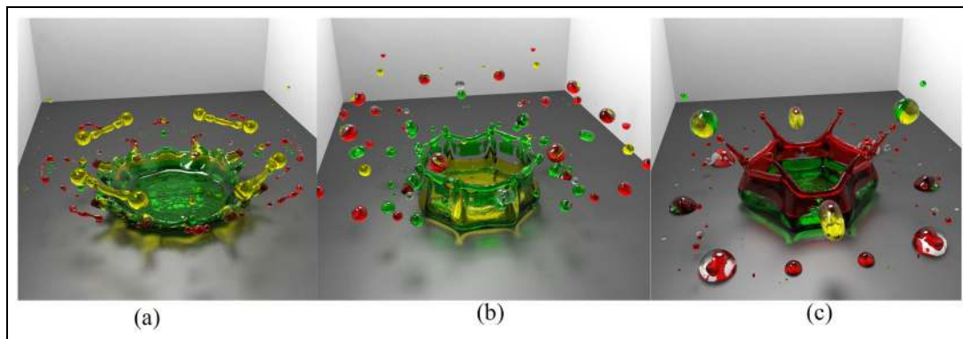
Figure 4. Results from the ethanol drop train impingement simulations at (a) u = 19 , T = 2.588 , (b) u = 22 , T = 6.276 and (c) u = 25 , T = 8.202 . The dimensionless times were selected only to highlight exemplary lamella formation. In all simulations lamella instability leads to secondary droplet ejection, classifying the impingement outcome as splashing.
