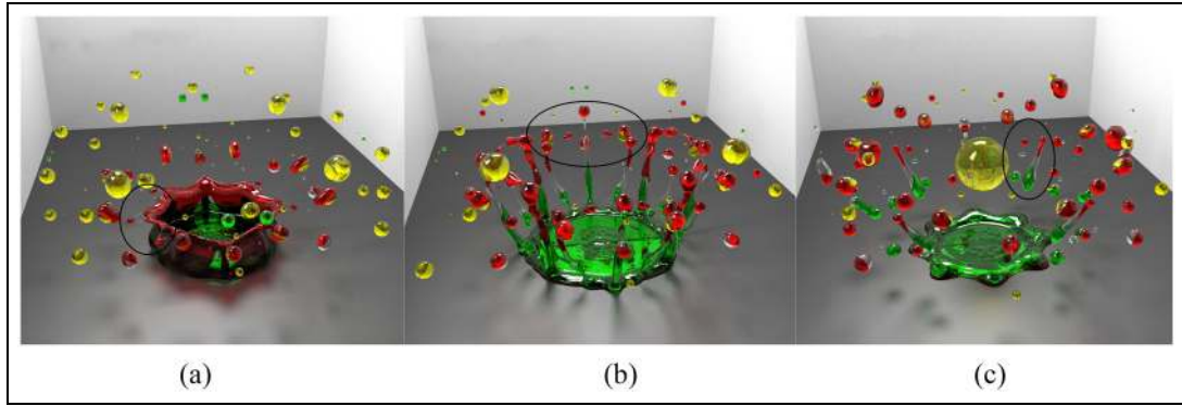
Figure 5. Results from the ethanol drop train impingement at u = 22 for three dimensionless times: (a) first phase of secondary droplet ejection where small droplets are ejected from lamella cusps ( T = 5.172 ). (b) Second phase of droplet ejection after the formation of ligaments at cusp locations ( T = 5.517 ). Larger secondary droplets are ejected from jets at the top of the ligaments. (c) Third phase of droplet ejection when the ligaments fracture into droplets of many sizes ( T = 5.862 ). Note the large yellow drop is the seventh drop of the drop train moving toward the surface before impinging.
