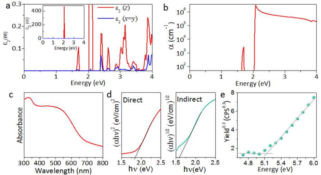
Figure 3. a) Calculated imaginary part of dielectric function. Inset: the view with larger scale of y-axis. b) Simulated optical absorption coefficient \alpha_z . c) Absorption spectra for the MDI single crystals. d) Tauc plots showing the direct and indirect nature of MDI bandgap. e) PESA measurement showing VBM at -5.11 eV for MDI.
